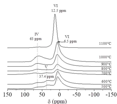
Figure 6: Variation of ^{27}\text{Al} NMR spectra as a function of the calcination temperature.
