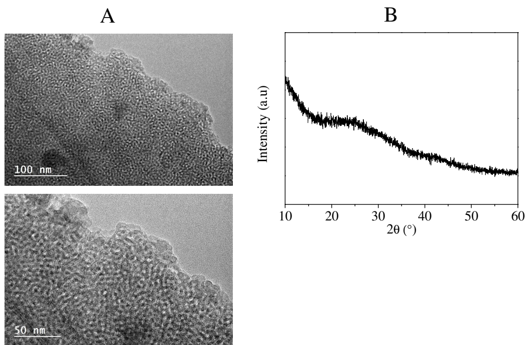
Figure S5: TEM images (A) and XRD (B) of the mesostructured alumina obtained after surfactant extraction by Soxhlet.
