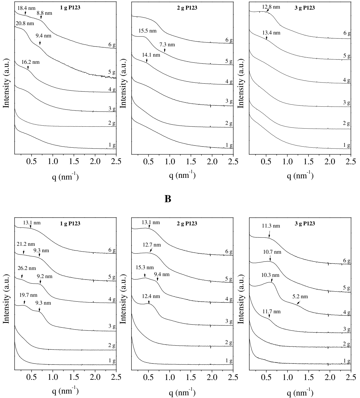
Figure S1: Evolution of the SAXS pattern as a function of the amount of both P123 and aluminum tri sec butoxide. Materials have been prepared without addition (A) or in the presence (B) of citric acid.
