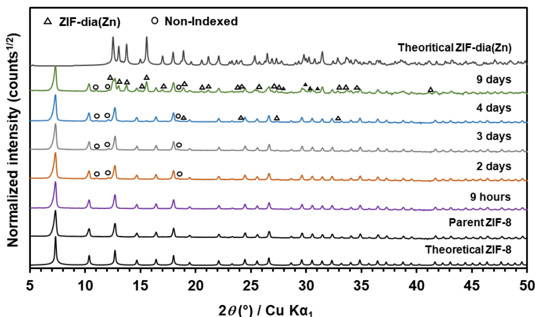
Figure 3. XRD patterns of simulated ZIF-8 and ZIF-dia (Zn), parent pellet sample, samples recovered after water intrusion–extrusion tests of different duration after 9 h and 2, 3, 4, and 9 days. Marks \Delta correspond to ZIF-dia(Zn) and marks \circ highlight non-indexed peaks for conventional ZIF-8 unit-cell.
