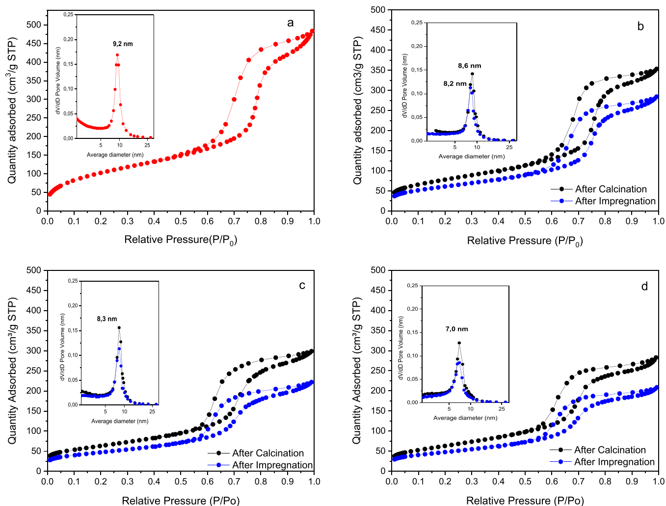
Figure 3. Nitrogen adsorption–desorption isotherm with the corresponding pore size distribution for (a) amorphous \text{TiO}_2 , (b) \text{TiO}_2 -300, (c) \text{TiO}_2 -340, and (d) \text{TiO}_2 -380.
